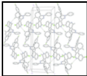
Fig. 2. The crystal packing of (I), showing extended one-dimensional chains along the c axis. H atoms not involved in the intermolecular interactions (dashed lines) have been omitted for clarity.
